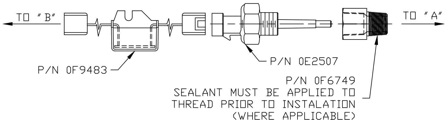
MECHANICAL DIAGRAM FOR NEW COOLANT LEVEL SENSOR INSTALATION
