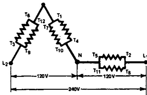
Figure 2.3-F. The 12-Lead Zig Zag System
