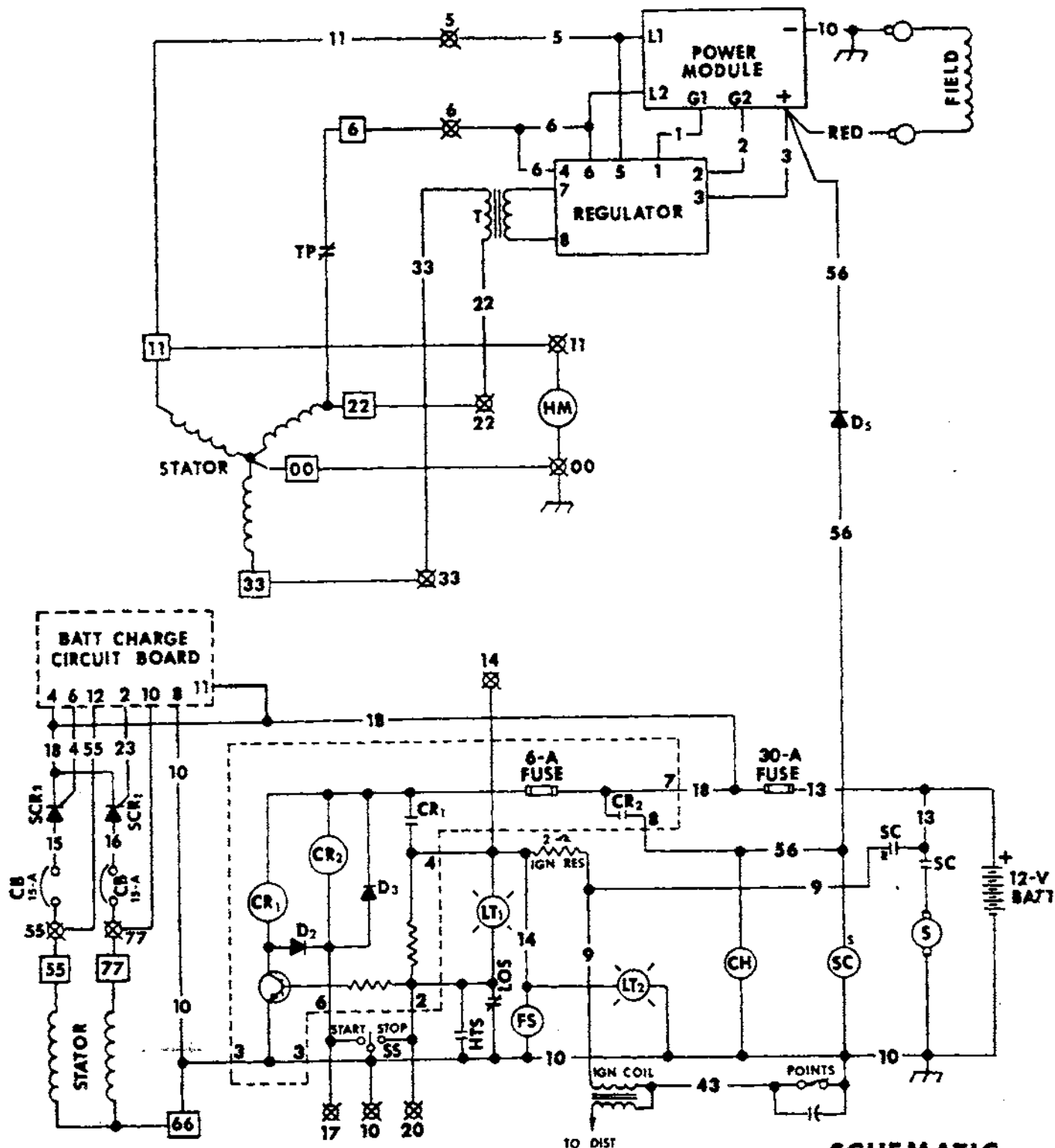
SCHEMATIC 46777
