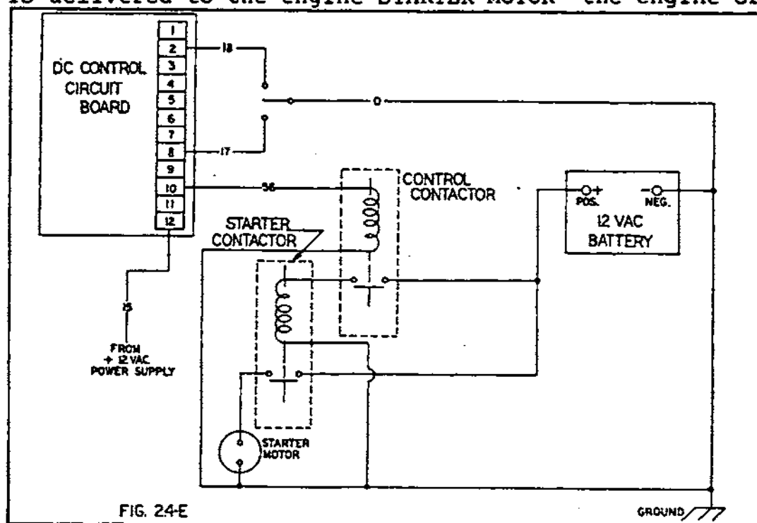
Figure 2.4-E. Typical Engine Cranking Circuit (Option "A" Units)
