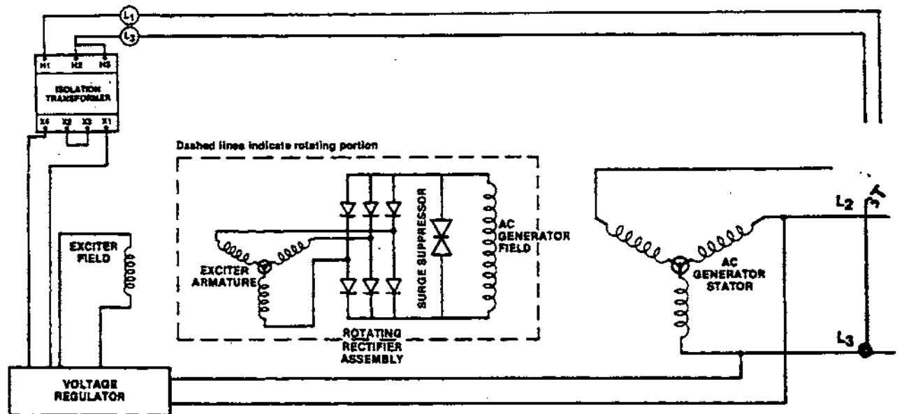
Figure 2.2-D. Block Diagram of Brushless AC Generator without a DPE Winding
