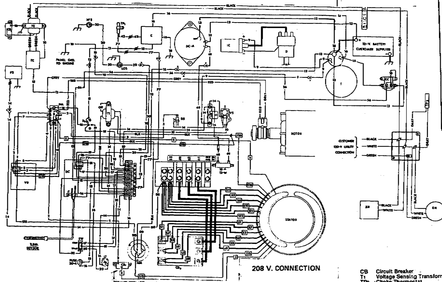
WIRING DIAGRAM No. 51101
