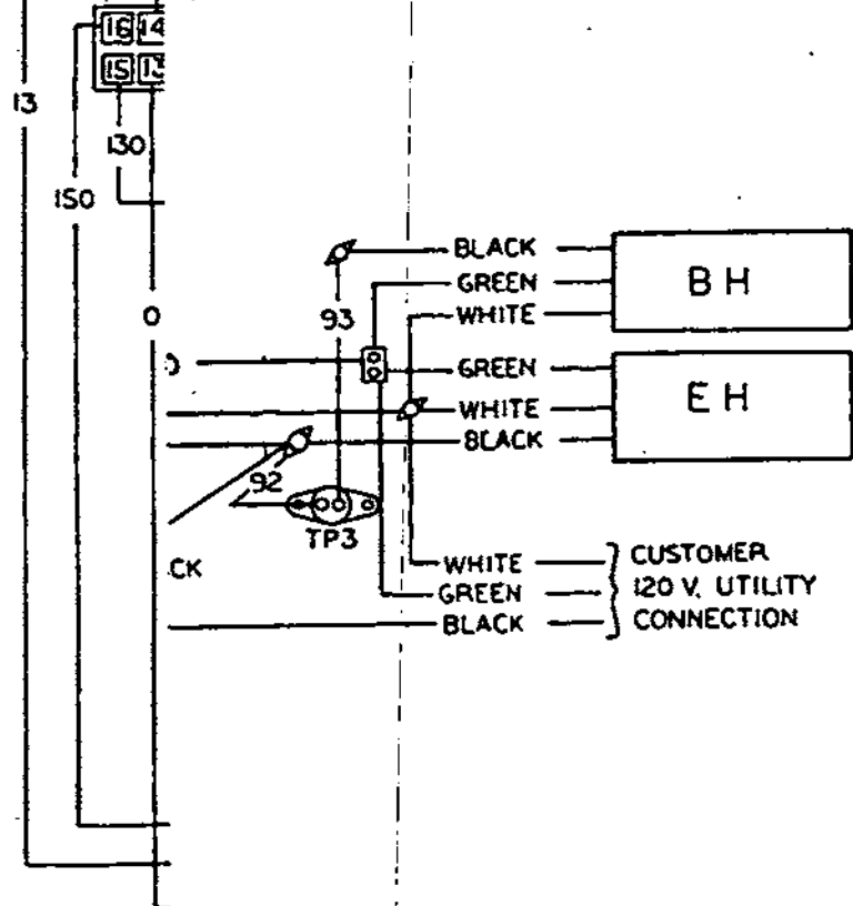
ENGINE WIRING DIAGRAM Drawing No. 58921
